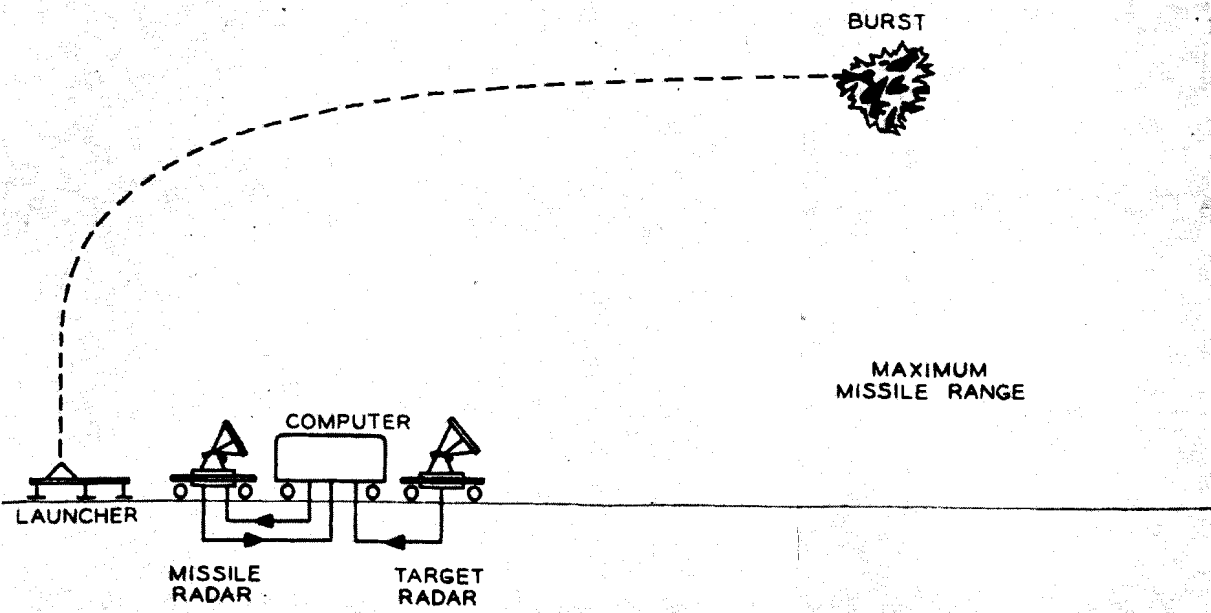
Figure 19. System Operation Phases—Pre-Launch, Turn, Steering, and Burst.
