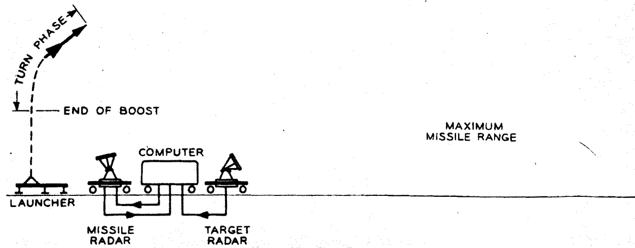
Figure 19. System Operation Phases—Pre-Launch, Turn, Steering, and Burst.
