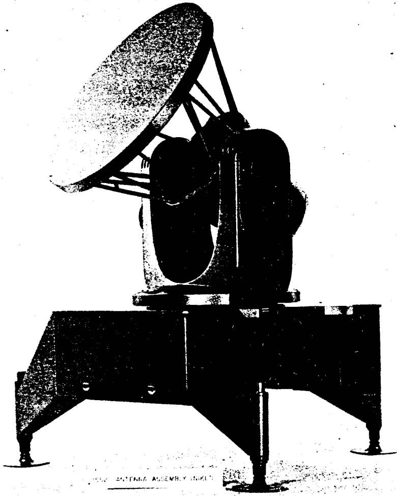
Figure 30. Tracking Antenna Assembly (BTL, 1 Oct 51)
