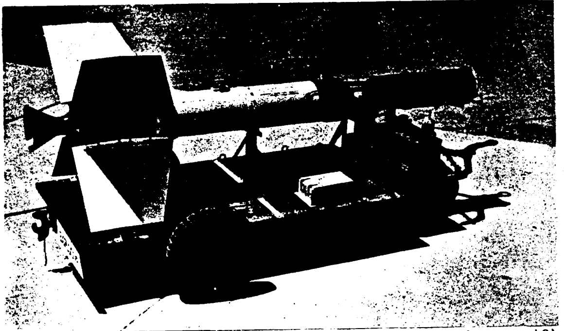
Figure 8. Single-Unit Booster Assembly on Handling Dolly (WSPG, 1948)
