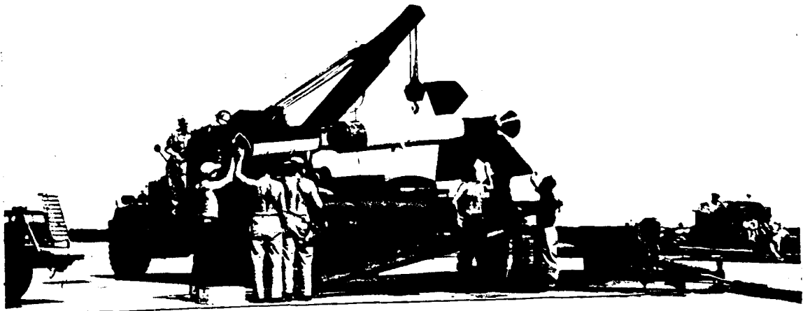
Figure 9. Loading Single Booster into Launcher No. 3 (WSPG, 1948)
