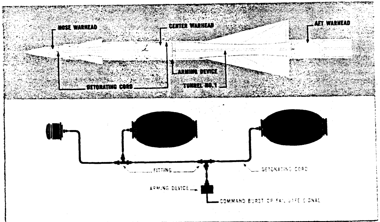
Figure 15. Warhead System
